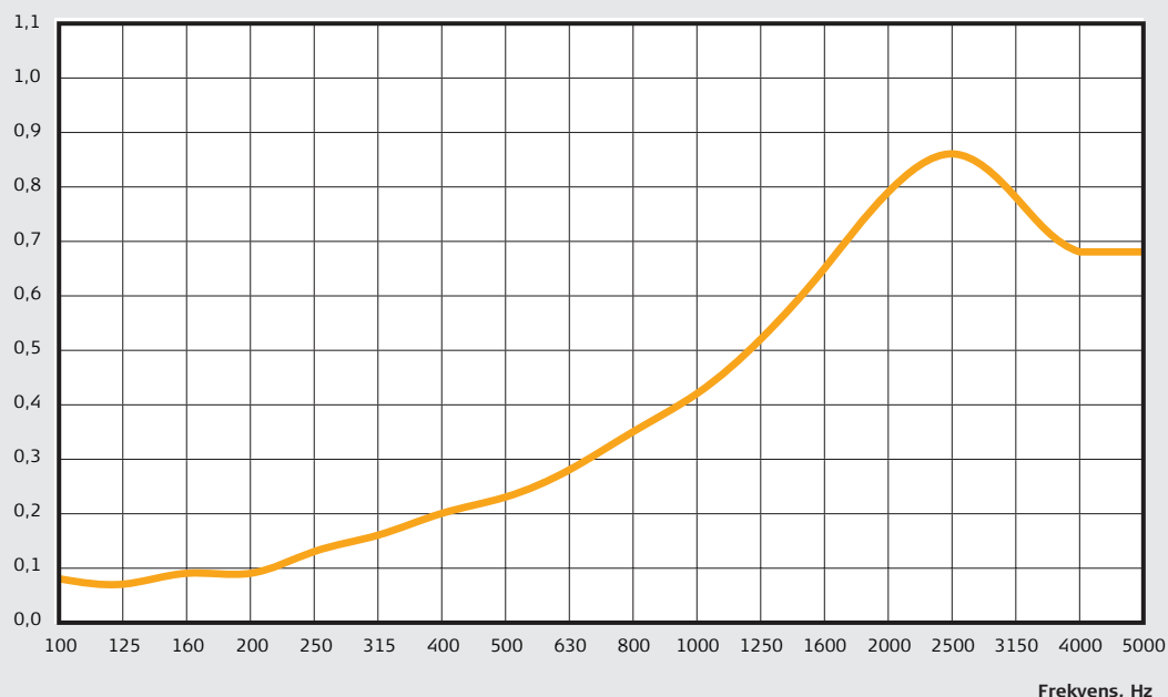
Absorptionskoefficient \alpha
