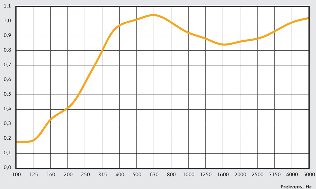
Absorptionskoefficient \alpha
